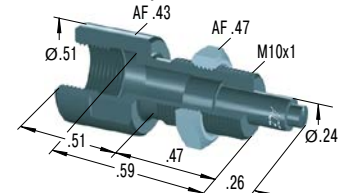
250-0562 Side Load Adaptor
