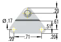
OA5-V4A Side Bracket
