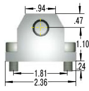
ME14 Bearing Shoe
