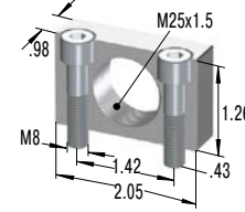
250-0436 Mounting Block
