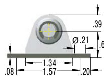
NG5-V4A Angle Bracket
