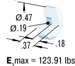
250-0753 Nylon Button
