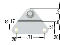
OG5-V4A Side Bracket
