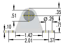
MA5-V4A Bearing Shoe
