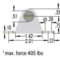
MA8-V4A Bearing Shoe
