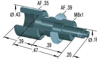
250-0141 Side Load Adaptor
