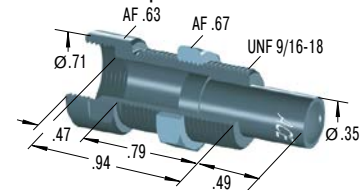
250-0554 Side Load Adaptor
