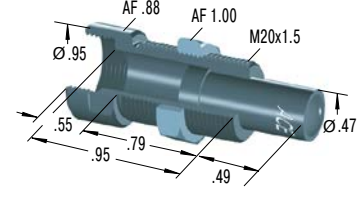
250-0559 Side Load Adaptor
