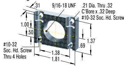
250-0318 Mounting Block
