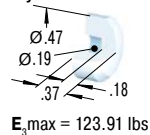
250-0753 Nylon Button
