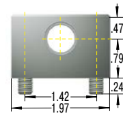
ND14 Mounting Flange
