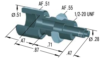
250-0762 Side Load Adaptor
