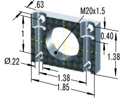
250-0353 Mounting Block
