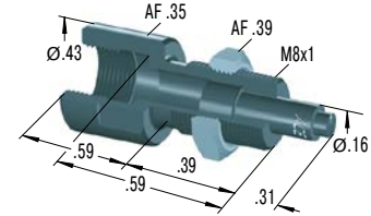
250-0146 Side Load Adaptor
